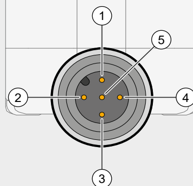
Emitter M12 Circular Connector Straight 5 PIN
